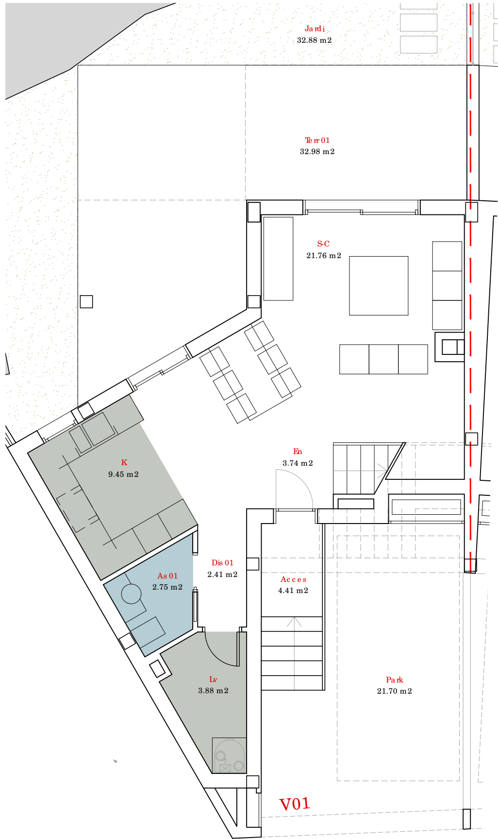
Ground floor
